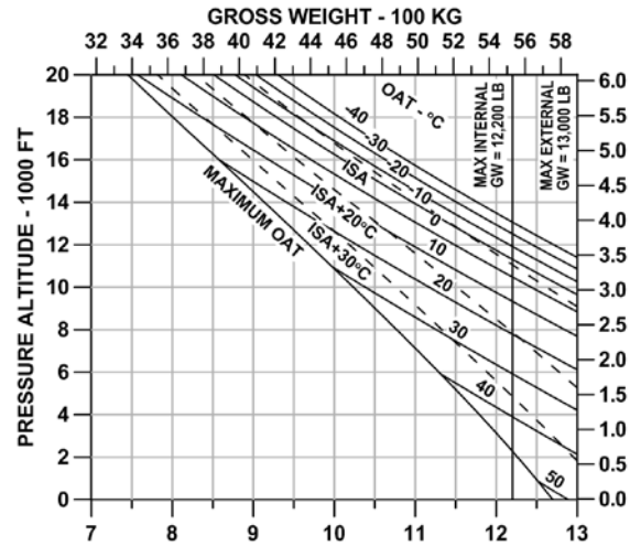
FAA Takeoff and Landing Limitation (WAT)
