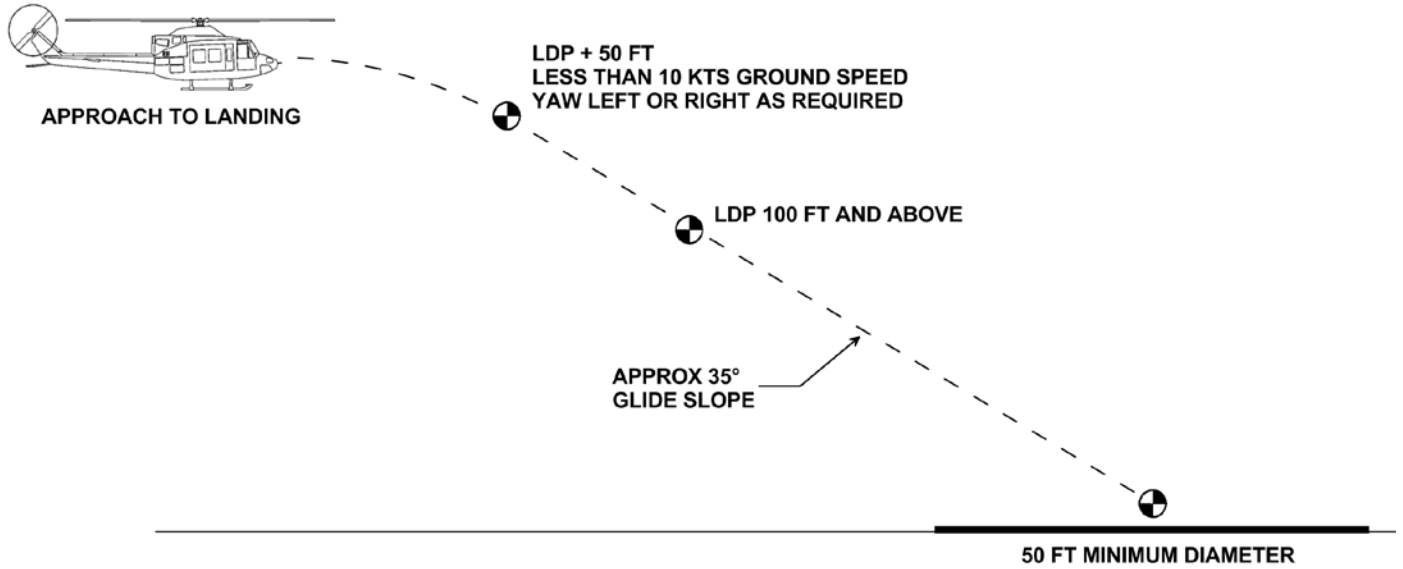
Normal landing (AEO) all engines operating
